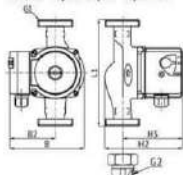
UPC 25-40, 25-60, 32-40, 32-60
