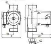
UPC 25-80, 32-80
